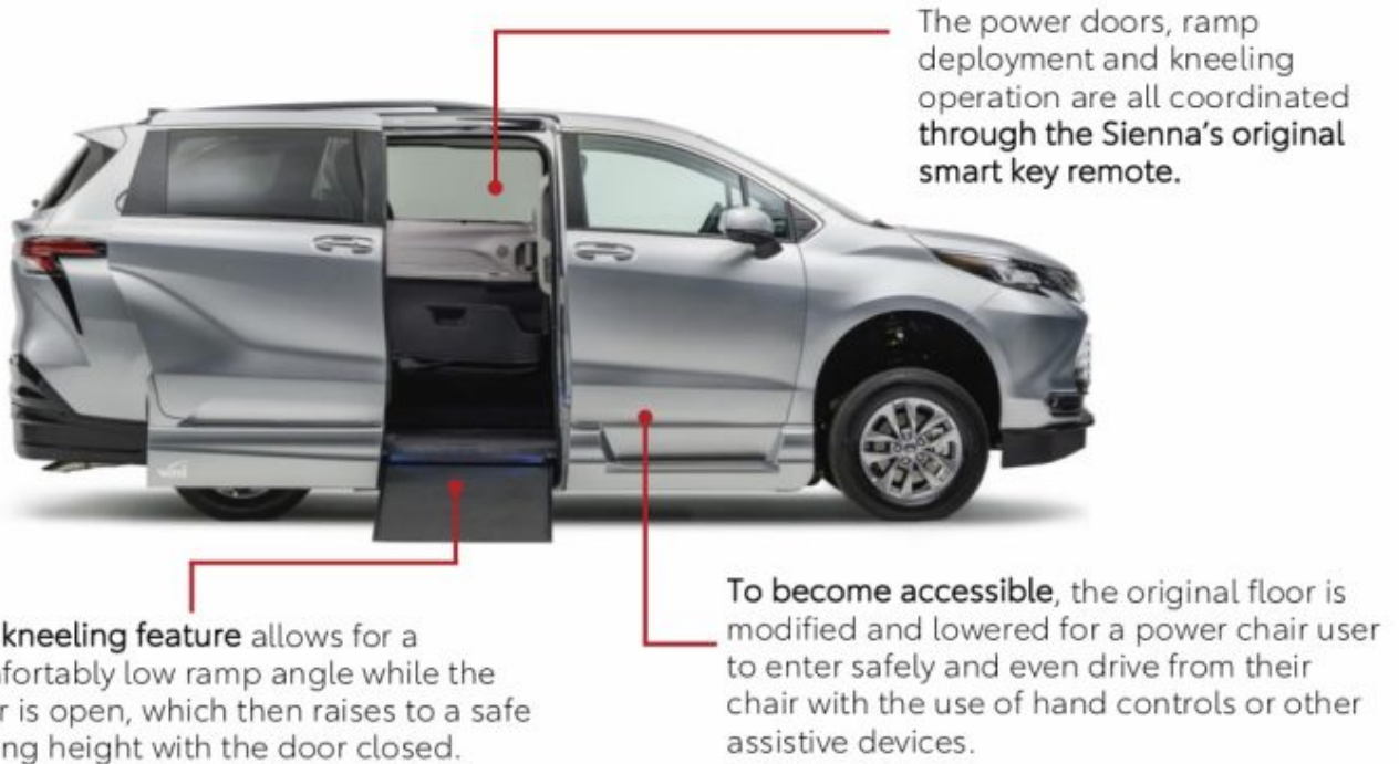
(Shown above: 2021 Sienna prototype shown with (VMI) Northstar conversion)
